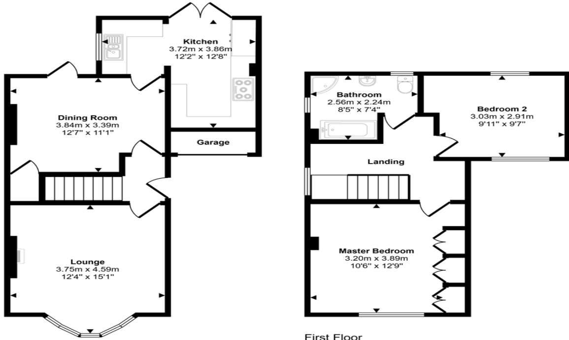
First Floor Approx 39 sq m / 416 sq ft
