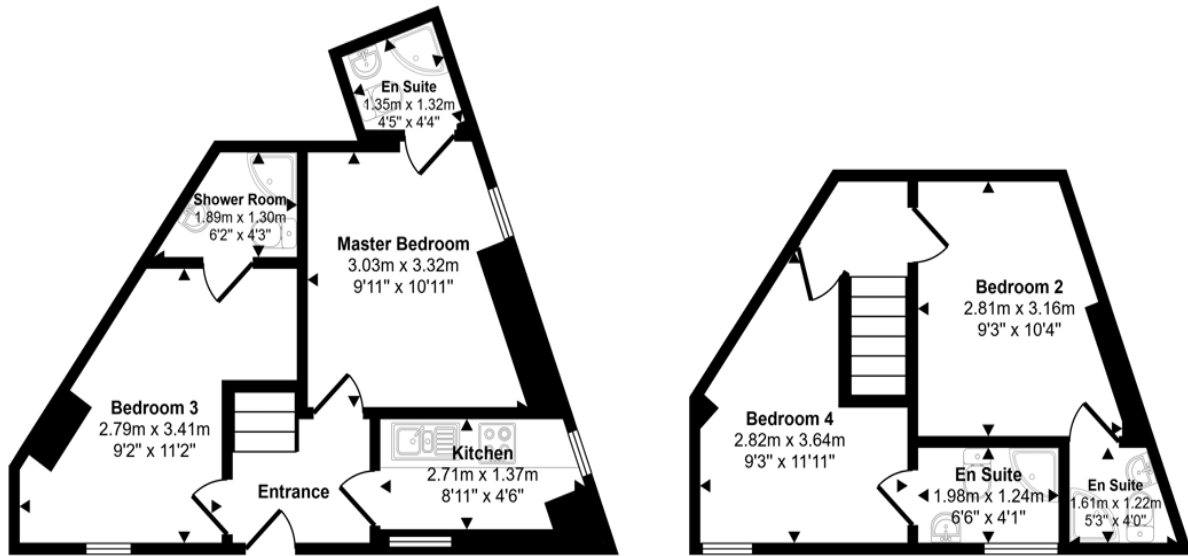
Ground Floor Approx 32 sq m / 341 sq ft
